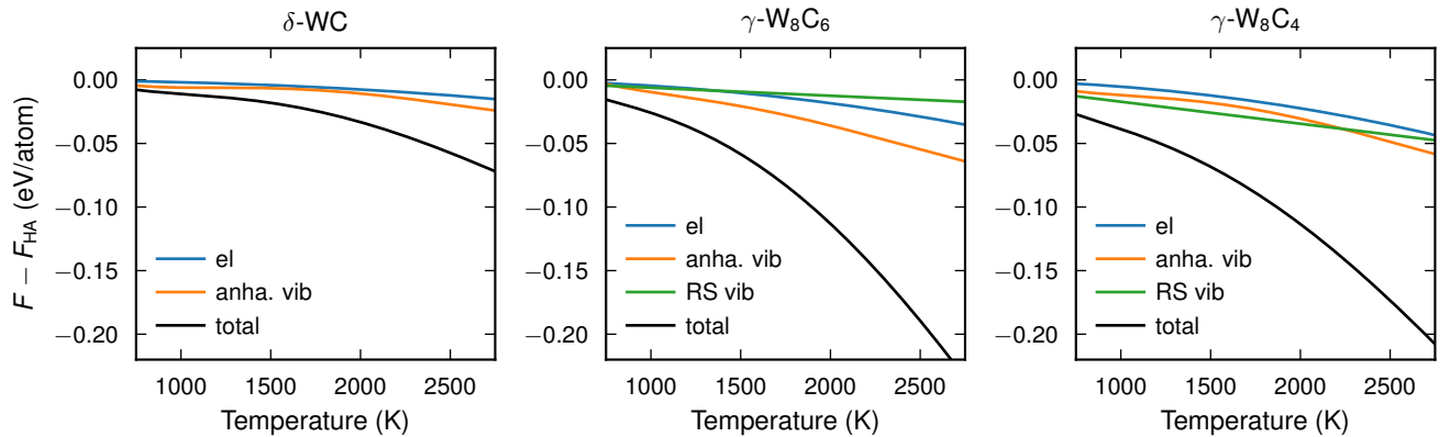
FIG. S10. Free energy contributions compared to free energy for ground-state structures using HA for two cases of sub-stoichiometric \gamma -WC: \gamma -W 8 C 4 (right) and \gamma -W 8 C 6 (middle), and the stoichiometric \delta -WC (left). The blue line (el) indicates the effect from electronic free energy and the orange line (anha. vib) indicates the effect from anharmonicity from EHMs. The green line (RS vib) indicates the vibrational free energy difference between disordered high-temperatures representative structures and ground states. The black line (total) indicates the difference between the total free free energy including thermal expansion and a HA.
