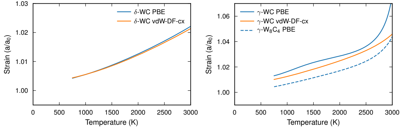
FIG. S9. Thermal expansion for stoichiometric \delta -WC (left) and \gamma -WC (right) computed with EHMs using both PBE and vdW-DF-cx. Also included is the thermal expansion for the sub-stoichiometric \gamma -W 8 C 4 ground state using PBE (right). The thermal expansion is shown as the lattice parameter relative to the relaxed lattice parameter at 0 K disregarding zero-point motion, a_0 . For the cubic phase we have a_{0,\text{PBE}}=4.378 Å and a_{0,\text{vdW-DF-cx}}=4.362 Å. For the hexagonal phase we have a_{0,\text{PBE}}=2.919 Å and a_{0,\text{vdW-DF-cx}}=2.905 Å. The sub-stoichiometric \gamma -W 8 C 4 ground state has a_{0,\text{PBE}}=4.212 Å. The expansion of the hexagonal crystal structure is done with a fixed c over a ratio: c/a = 0.9747 .
