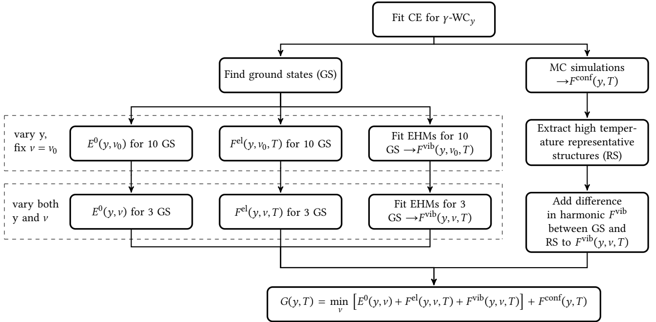
FIG. S1. Workflow diagram for calculating the free energy of \gamma -WC, i.e., cubic WC. Here, \nu_0 is the relaxed specific volume.
