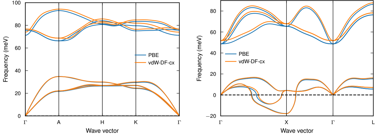
FIG. S6. The harmonic (0 K) phonon dispersions for stoichiometric \delta -WC (left) and \gamma -WC (right) in the HA using both PBE and vdW-DF-cx.
