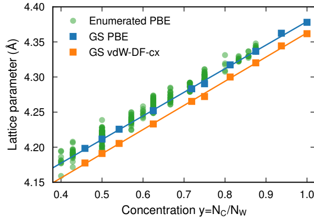
FIG. S8. The effective lattice parameter for relaxed, i.e. disregarding zero-point motion, 0 K \gamma -WC ground states (GSs) as a function of carbon concentration computed with both PBE and vdW-DF-cx exchange-correlation functionals. The ground states are found through simulated annealing simulations using the CE for \gamma -WC. The solid lines are linear fits to the discrete data points (squares). Also included are the effective lattice parameters of relaxed enumerated structures calculated using PBE.
