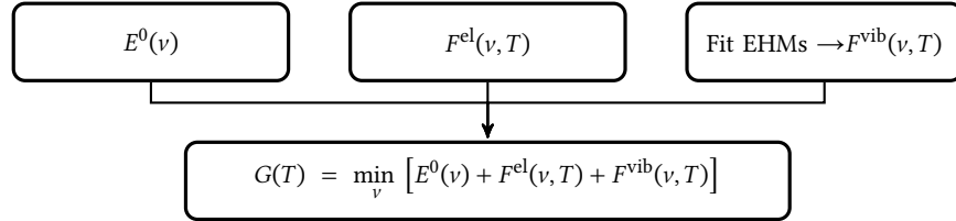
FIG. S4. Workflow diagram for calculating the free energy of BCC-W.
