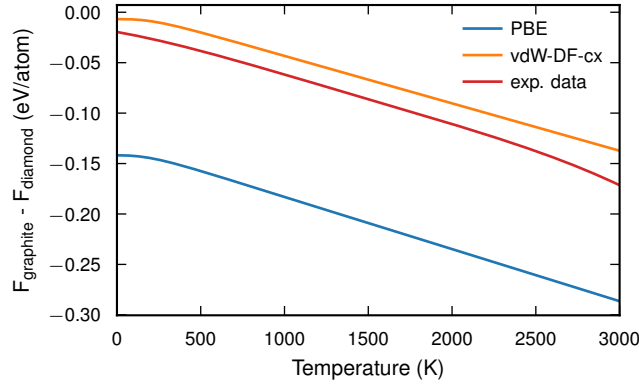
FIG. S7. Difference in free energy between graphite and diamond using HA with either PBE or vdW-DF-cx compared to the value using experimental data from Refs 1 and 2. The HA used are the same as Fig. S5.
