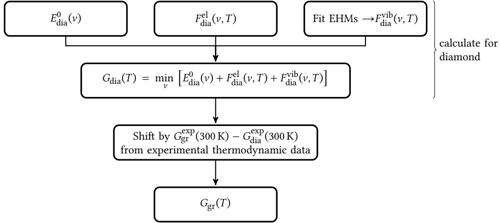
FIG. S3. Workflow diagram for calculating the free energy of graphite. Experimental data taken from Refs. 1 and 2.
