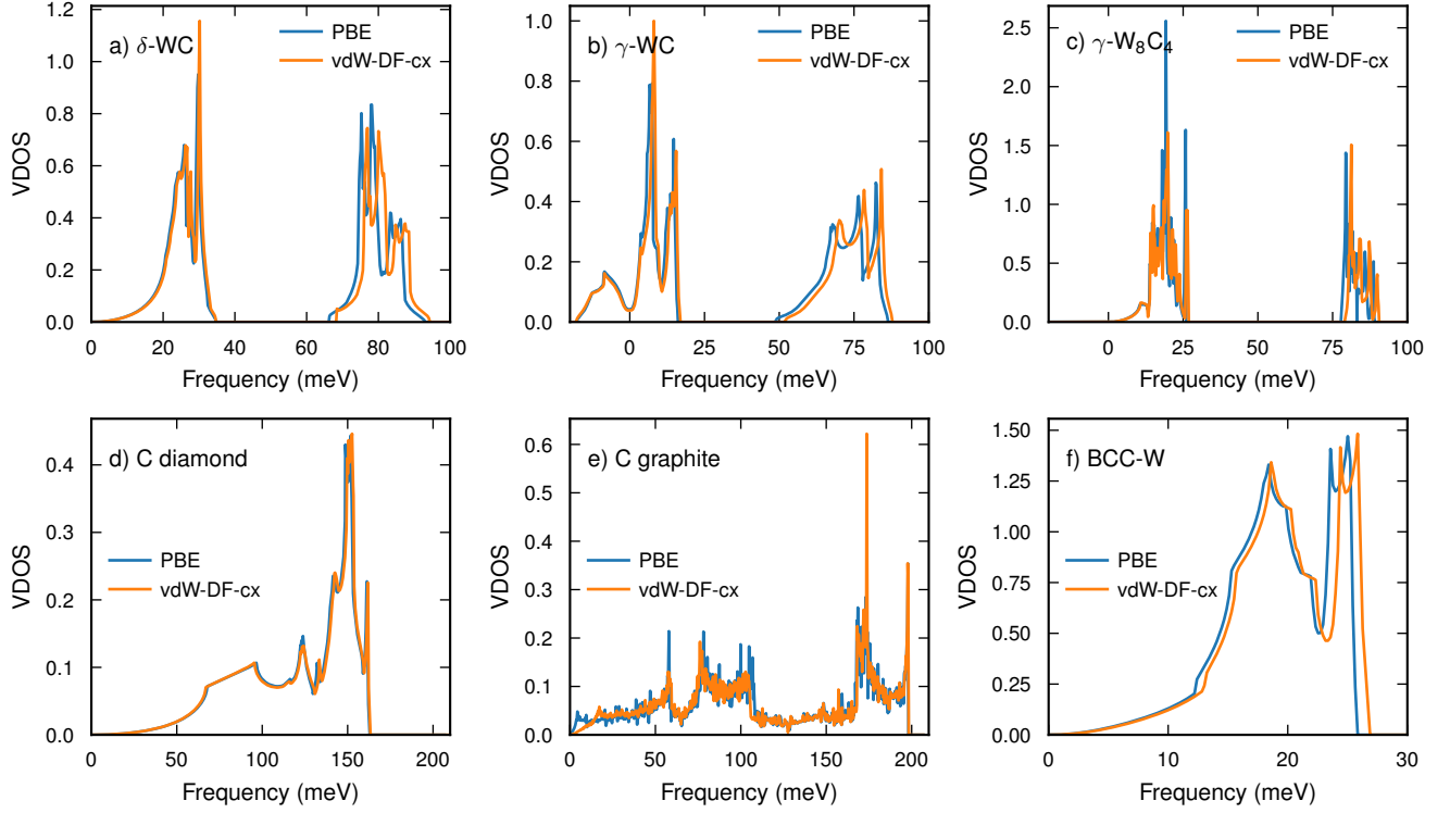
FIG. S5. The harmonic (0K) VDOS for stoichiometric \delta -WC and \gamma -WC, the ground state configuration for the sub-stoichiometric \gamma -W 8 C 4 , diamond, graphite and BCC-W. Results using both PBE and vdW-DF-cx are shown.
