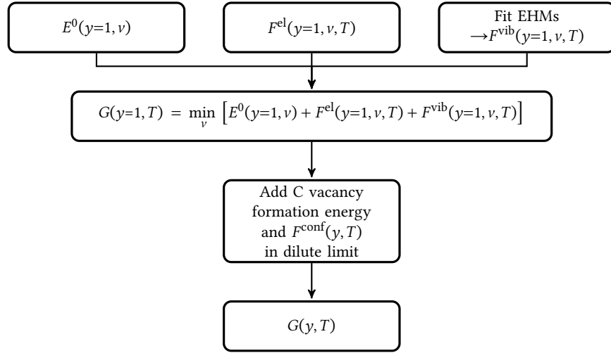
FIG. S2. Workflow diagram for calculating the free energy of \delta -WC, i.e., hexagonal WC.
