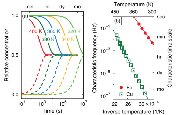
FIG. 6. (Color online) Vacancy redistribution in the presence of an oscillating external field: (a) Equilibration over vacancy types Cu_{Ti}-V_{c1} (solid lines) and Cu_{Ti}-V_{c2} (dashed lines) in the presence of an external oscillating field with a cycling frequency of 1 Hz for temperatures between 320 and 400 K. (b) Temperature dependence of time after which the relative concentration of M_B-V_{c1} complexes is reduced to 55% where M is either Cu or Fe.
