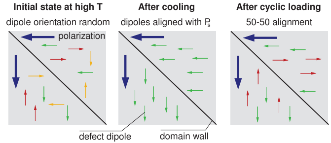
FIG. 8. (Color online) Schematic representation of defect dipole arrangements under different conditions as deduced from the kinetic model. The large value arrows indicate the matrix polarization in different domains while the small arrows represent defect dipoles. The thick solid line illustrates the position of a 90^\circ domain wall.
