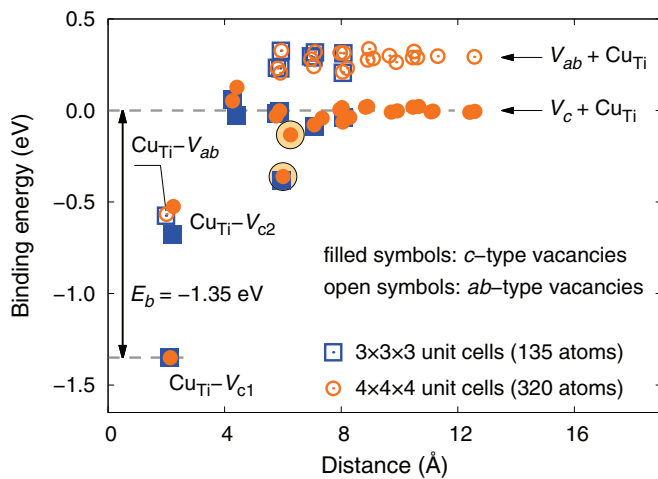
FIG. 2. (Color online) Binding energy of \text{Cu}_{\text{Ti}}\text{-V}_{\text{O}} complexes as a function of the distance between the Cu atom at the vacancy center. The gray horizontal line indicates the noninteracting limit. The two configurations marked by shaded circles correspond to third nearest neighbor impurity-vacancy complexes that are aligned along [001].
