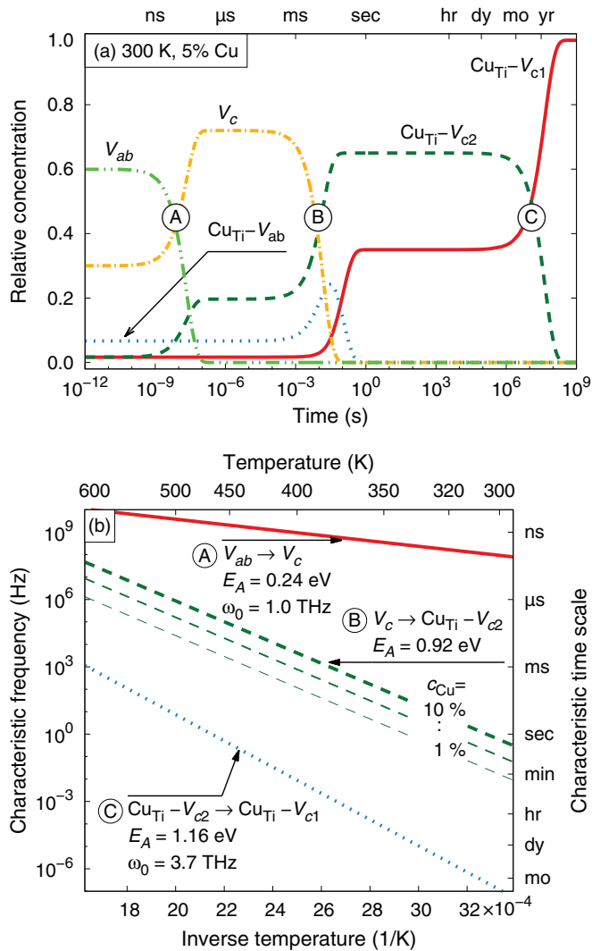
FIG. 5. (Color online) Vacancy redistribution in the absence of electric fields for Cu-doped lead titanate: (a) Temporal evolution of the relative concentrations of different vacancy types at a temperature 300 K and for a Cu concentration of 5%. (b) Temperature dependence of the characteristic transition times marked by white circles in (a). The transition time for the conversion from V_c to Cu_{Ti}-V_{c2} depends on the Cu concentration as exemplified by the three green dashed lines of varying thickness.
