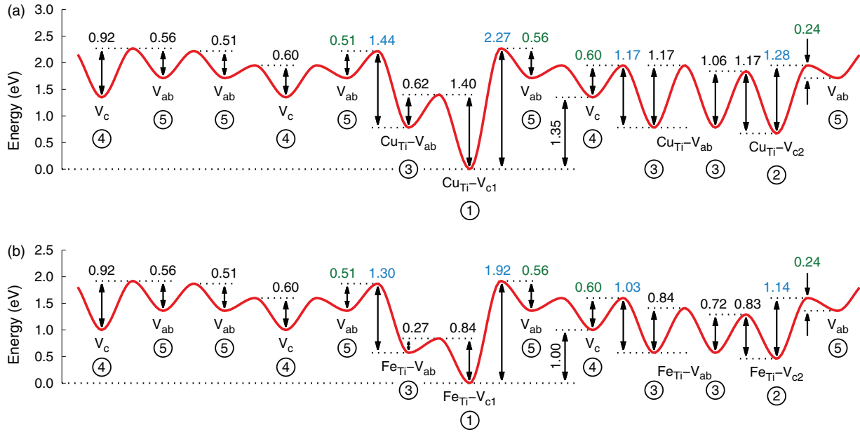
FIG. 4. (Color online) Energy surface for the migration of oxygen vacancies in (a) Cu-doped ( \text{Cu}_{\text{Ti}}\text{-V}_O , q = 0 ) and (b) Fe-doped \text{PbTiO}_3 ( \text{Fe}_{\text{Ti}}\text{-V}_O , q = +1 ). The sequence of barriers corresponds to a (hypothetical) continuous trajectory which illustrates all possible migration barriers (compare Figs. 1 and 3).
