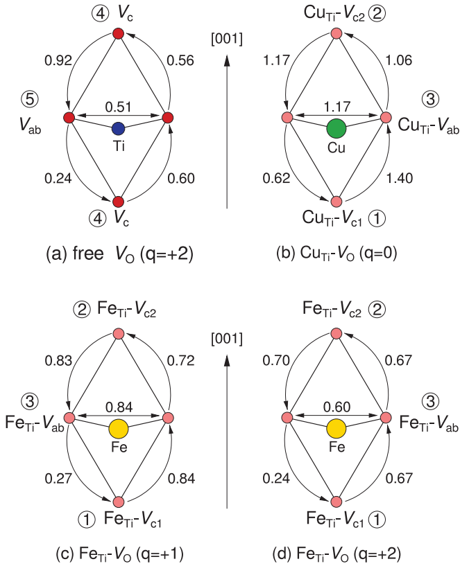
FIG. 3. (Color online) Schematic representation of the barriers for the migration of free (a) and complexed (b)–(d) oxygen vacancies in units of eV. Each figure shows the projection of a BO_6 octahedron onto the (100) plane. The numbers in circles indicate the indices used to distinguish the different processes. Oxygen sites (and thus possible vacancy sites) are shown as red circles while the position of the B -site cation (Ti, Cu, or Fe), which is situated at the center of the oxygen octahedron, is indicated by blue (Ti), green (Cu), and yellow (Fe) circles.
