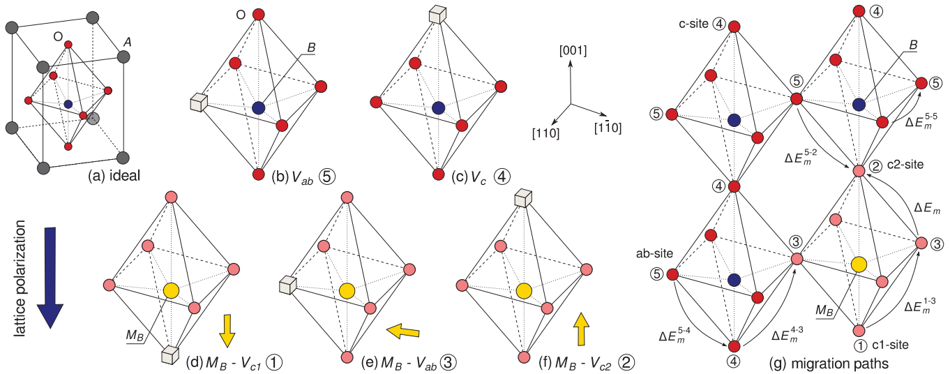
FIG. 1. (Color online) (a) Unit cell of the ideal tetragonal perovskite ( ABO_3 ) lattice. (b),(c) Free oxygen vacancies. (d)–(f) Complexed oxygen vacancies on nearest-neighbor sites of B -site impurities. The dark blue arrow on the left indicates the direction of the lattice polarization whereas the smaller yellow arrows represent the orientation of the defect dipoles. (g) Schematic representation of the possible paths for oxygen vacancy migration. Some migration barriers, \Delta E_m^{i-j} , are exemplarily indicated. In (b)–(g) only the B and O sites are shown. Oxygen vacancies jump along the vertices of the BO_6 octahedron. Blue and yellow circles represent native and impurity atoms on B sites, respectively. The dark and light red circles indicate oxygen atoms in the first nearest neighbor shell of native and impurity atoms, respectively.
